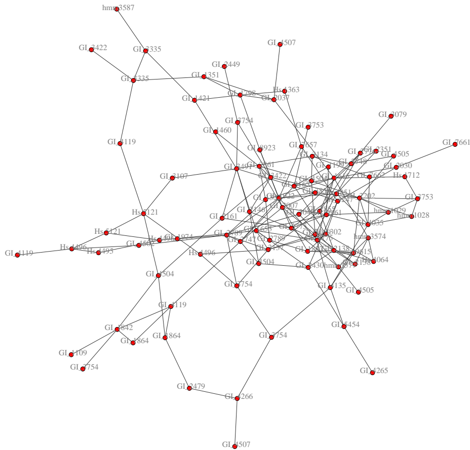
Figure 8: The inferred graph for the human gene expression dataset using Gaussian copula graphical models. This graph consists of 176 links with estimated posterior probabilities greater than 0.5.
