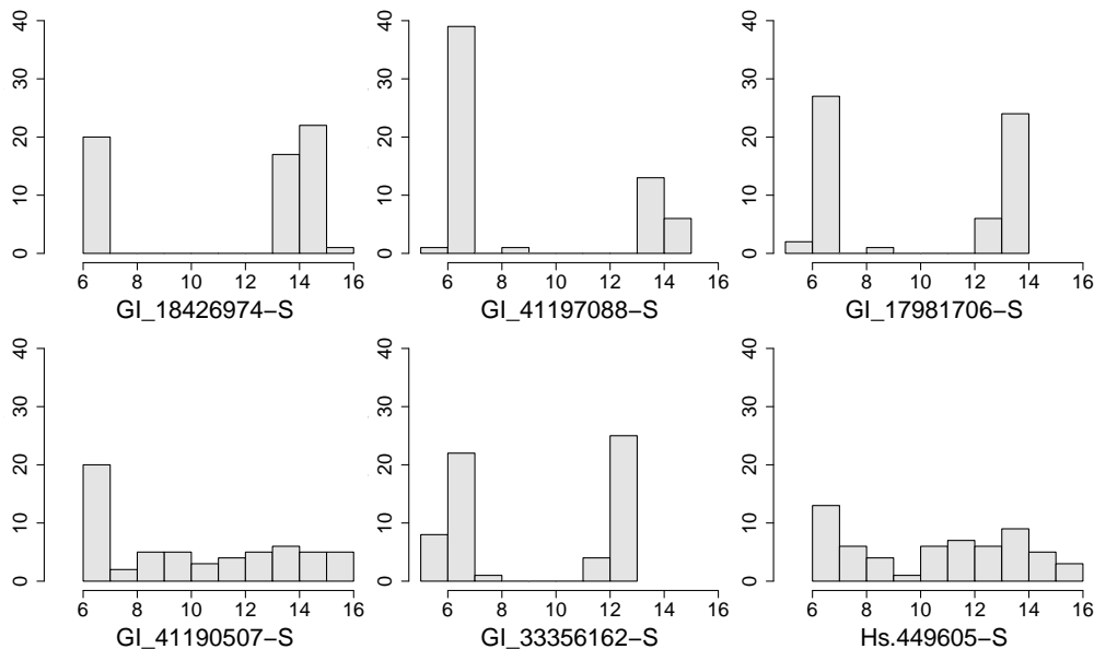
Figure 7: Univariate histograms of the first 6 genes in the human gene expression dataset.
