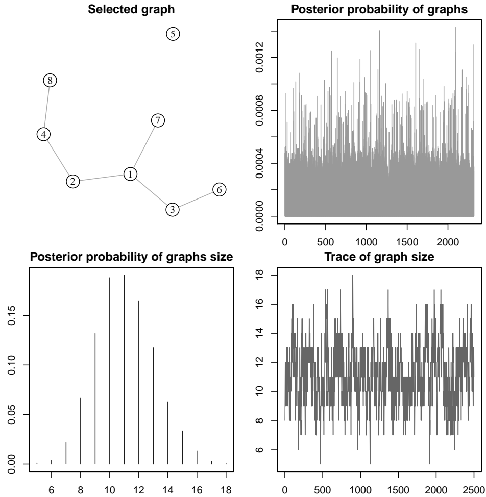
Figure 3: Visualization summary of simulation data based on output of the bdgraph function. The figure in the top-left is the inferred graph with the highest posterior probability. The figure in the top-right gives the estimated posterior probabilities of all visited graphs. The figure in the bottom-left gives the estimated posterior probabilities of all visited graphs based on the size of the graphs. The figure in the bottom-right gives the trace of our algorithm based on the size of the graphs.
