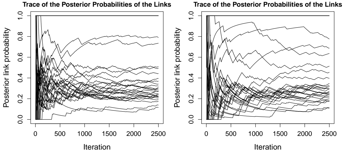
Figure 5: Plot for monitoring the convergence based on the trace of the estimated posterior probability of all possible links for the BDMCMC algorithm (left) and the RJMCMC algorithm (right).
