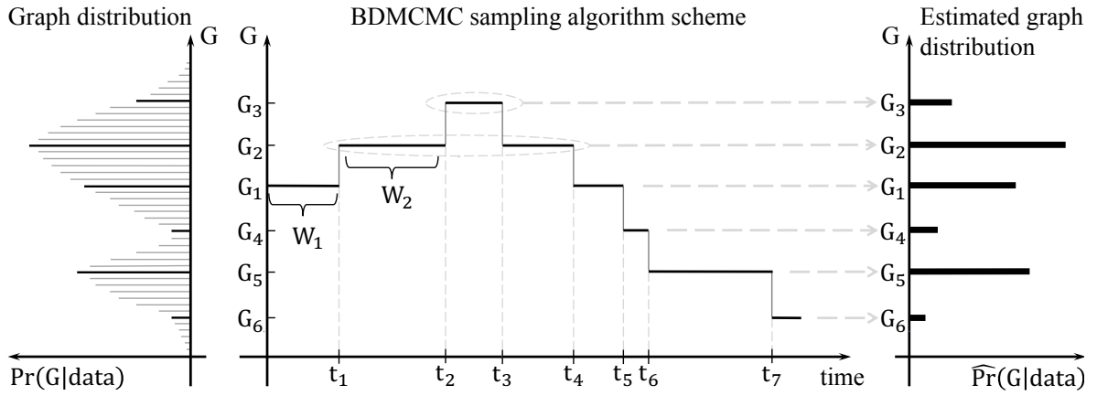
Figure 2: This image visualizes the Algorithm 2. The left side shows the true posterior distribution of the graph. The middle panel presents a continuous time BDMCMC sampling algorithm where \{W_1, W_2, \dots\} denote waiting times and \{t_1, t_2, \dots\} denote jumping times. The right side denotes the estimated posterior probability of the graphs in proportion to the total of their waiting times, according to the Rao-Blackwellized estimator.
