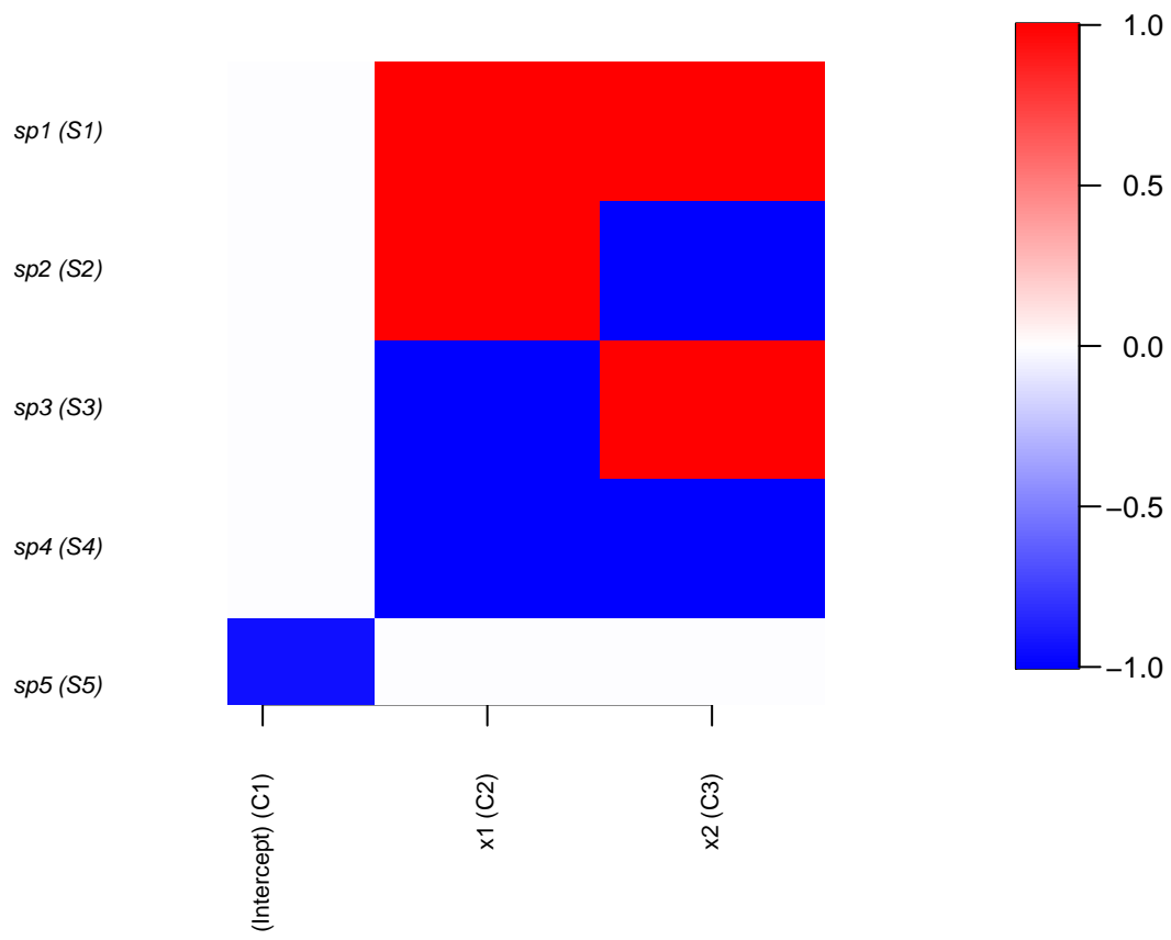
Figure 2: Heatmap of Beta parameters
